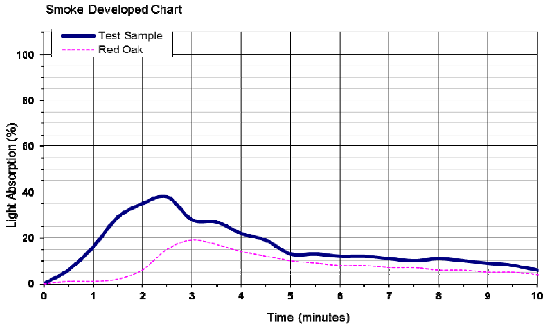
Figure 2 Smoke Developed Chart
